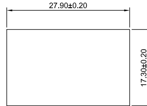
Panel Hole Layout
