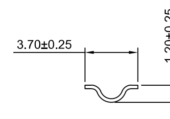
SEC:C-C
