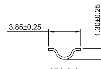
SEC:C-C
